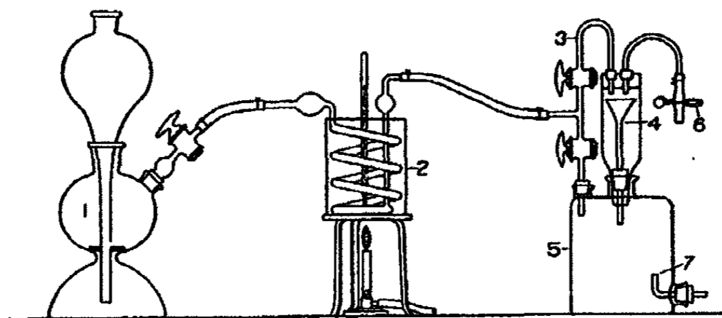
Apparatus for Filtering, Washing and Drying Boron Compounds
